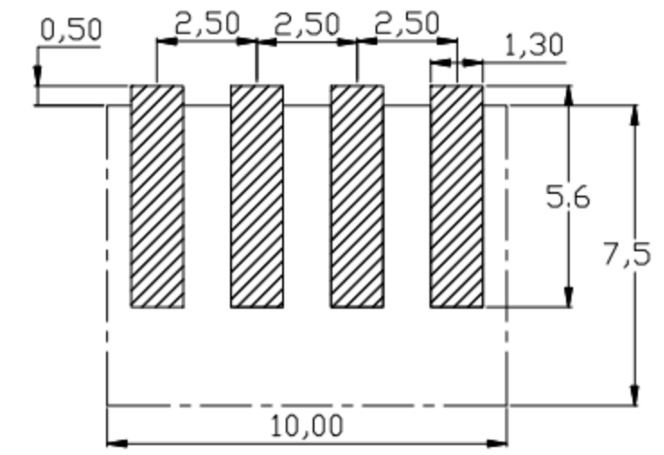
RECOMMENDED PCB LAYOUT TOP VIEW(.XX±0.05)
